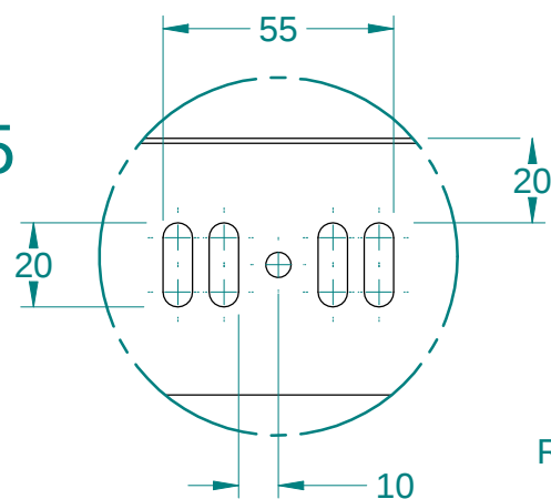
DETAIL A 1:2
